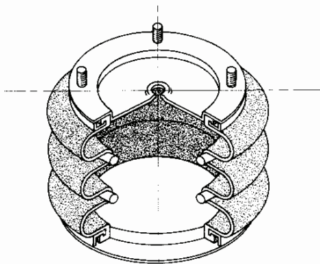
BELLOWS
