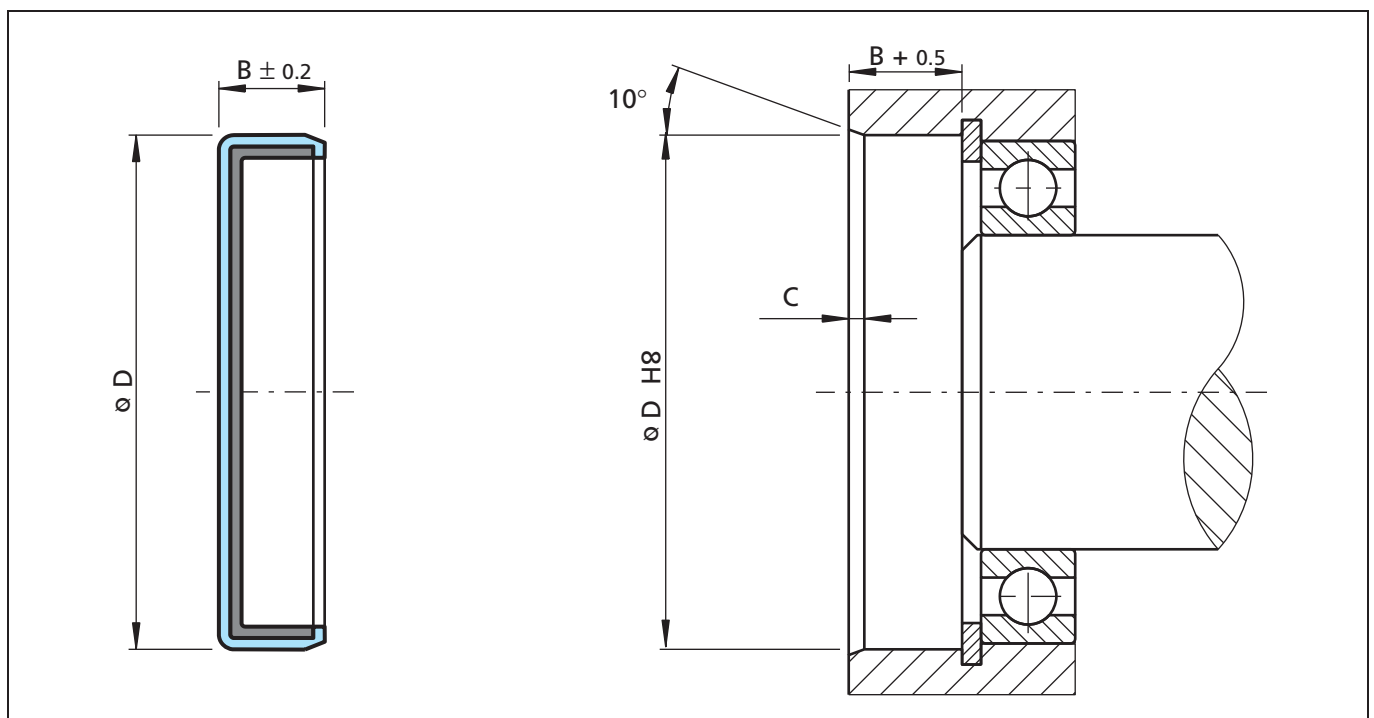
Figure 44 Installation drawing
