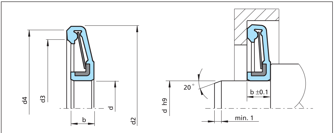
Figure 88 Installation drawing
