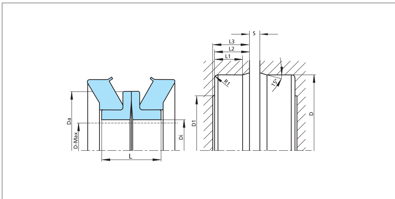
Figure 150 Installation Drawing
